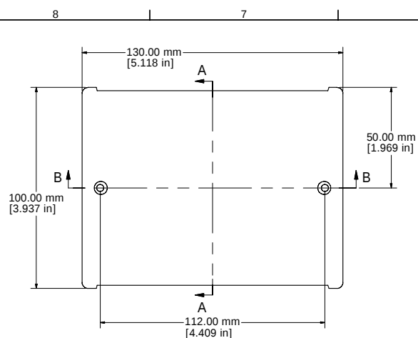
ASSEMBLY - BOTTOM
