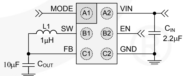
Figure 1. Typical Application
