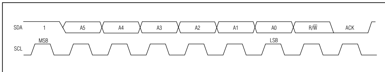
Figure 5. Slave Address
