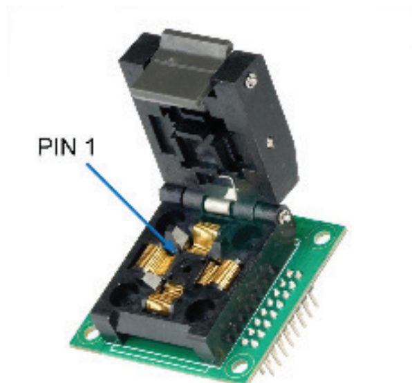
Figure 3.2 VPROG-1-S-LQFP48
