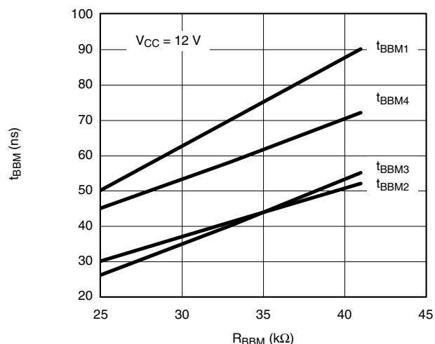
t_{BBM} vs. R_{BBM} , V_{EP} = 0\text{ V}
