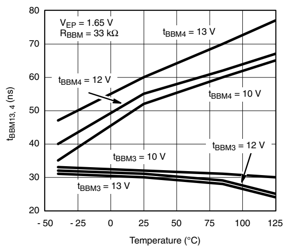
t_{BBM3,4} vs. Temperature, V_{EP} = 1.65\text{ V}
