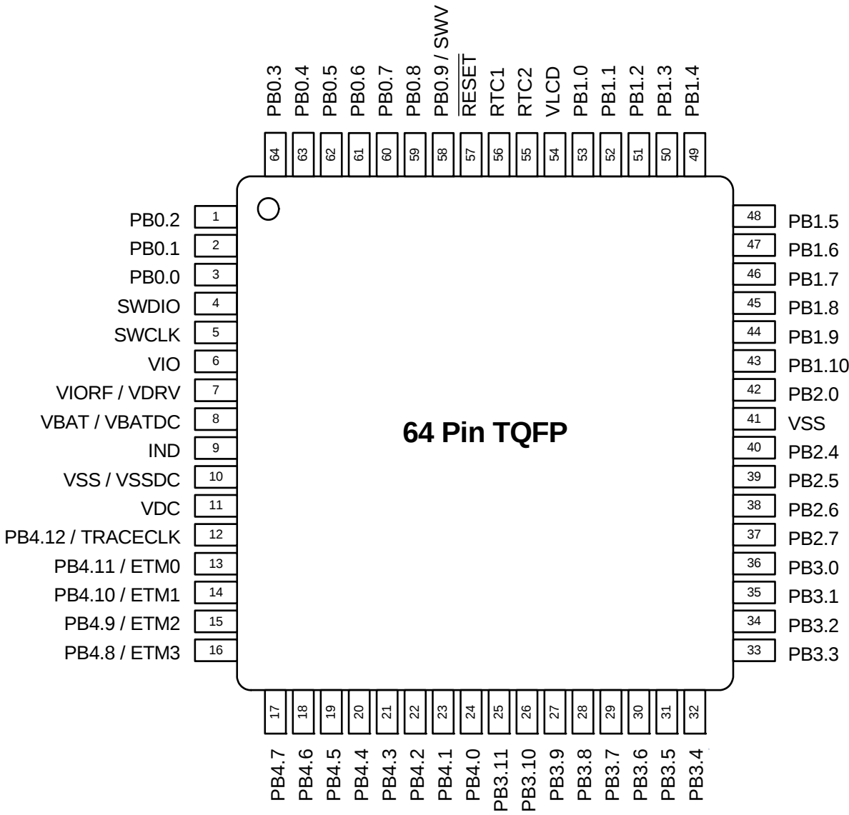
Figure 6.3. SiM3L1x6-QG Pinout
