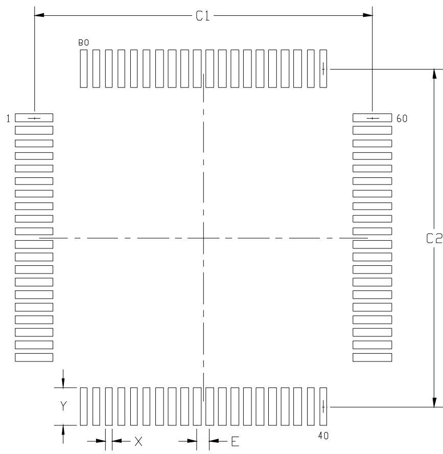
Figure 6.7. TQFP-80 Landing Diagram
