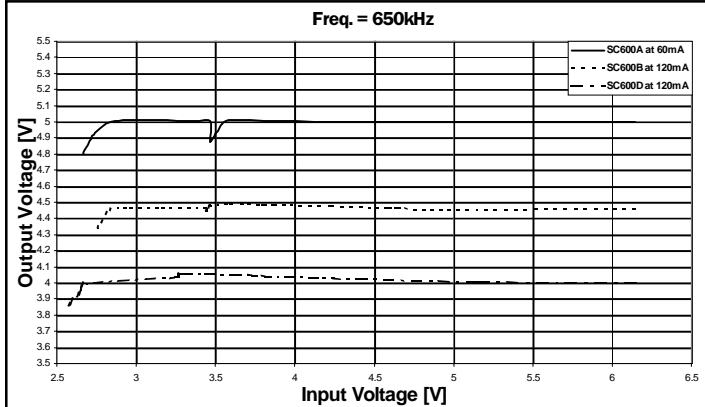
Line Regulation
