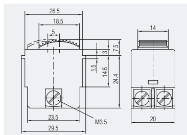
Screw connection M3.5 1205.0101
