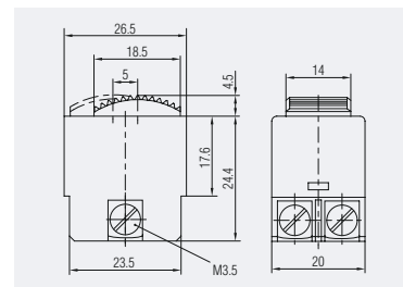
Screw connection M3.5 1205.0304 without collar
