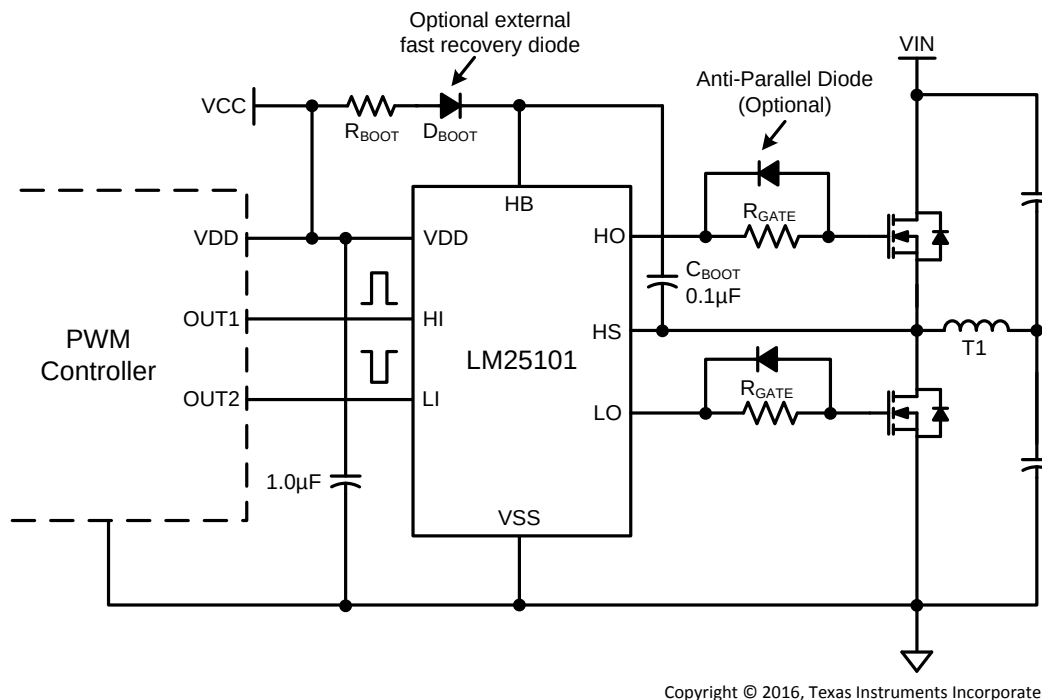
Figure 21. Application Diagram
