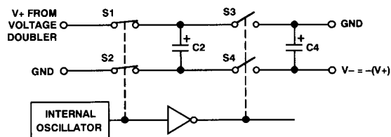
Figure 2. Voltage Inverter
