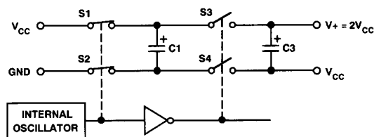
Figure 1. Voltage Doubler
