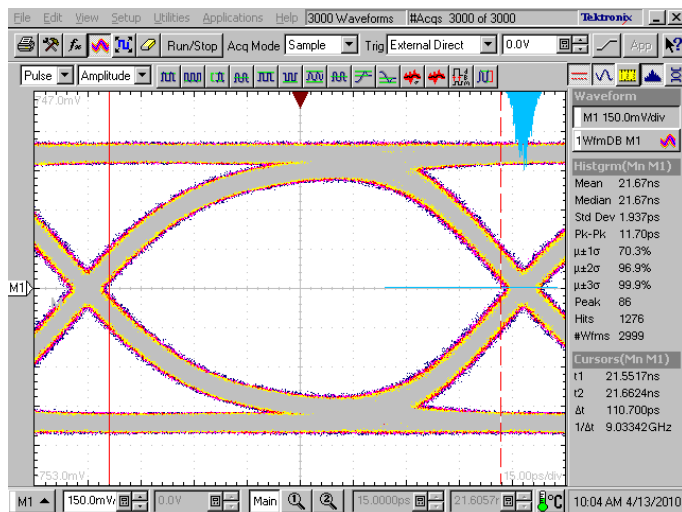
5.0 Gbps RX signal eye with PI3USB302-A
