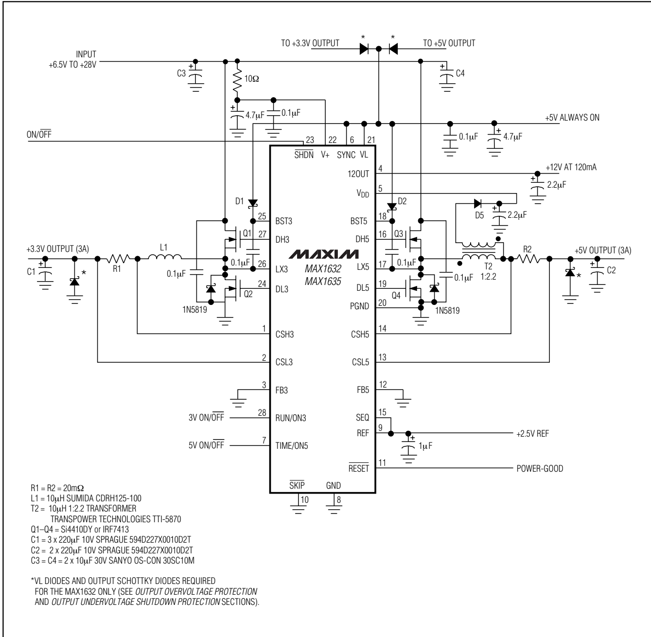
Figure 9. Triple-Output Application for High-Voltage Batteries (MAX1632/MAX1635)
