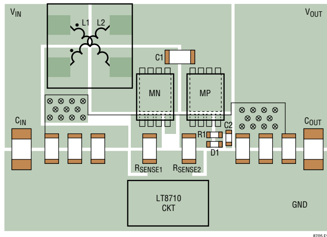
Figure 19. Suggested Component Placement for Dual Inductor Inverting Topology
