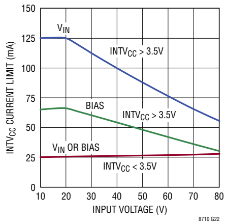
INTV CC Current Limit vs V IN or BIAS
