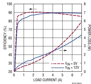
Efficiency and Power Loss
