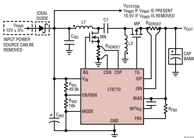
Figure 12. Backup Power Converter
