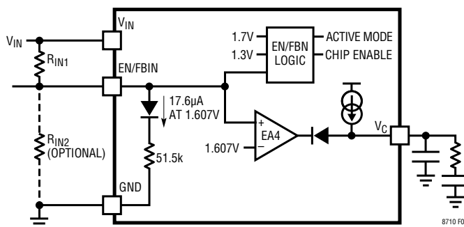
Figure 8. Configurable UVLO
