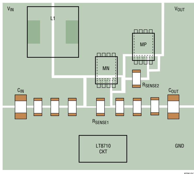
Figure 17. Suggested Component Placement for Boost Topology
