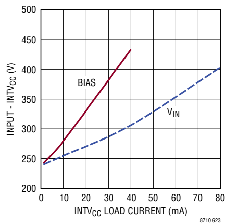
INTV CC Dropout from V IN or BIAS
