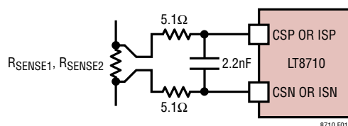
Figure 14a. Differential RC Filter on CSP/CSN and/or ISP/ISN Pins
