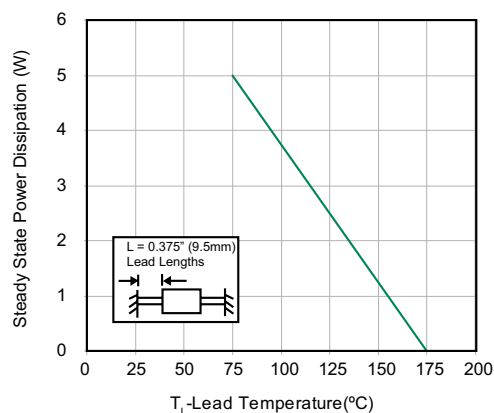
Figure 6 - Steady State Power Derating Curve
