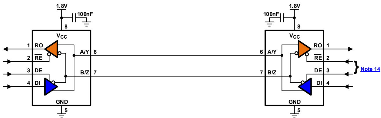
FIGURE 3. HALF DUPLEX NETWORK USING ISL32603E
