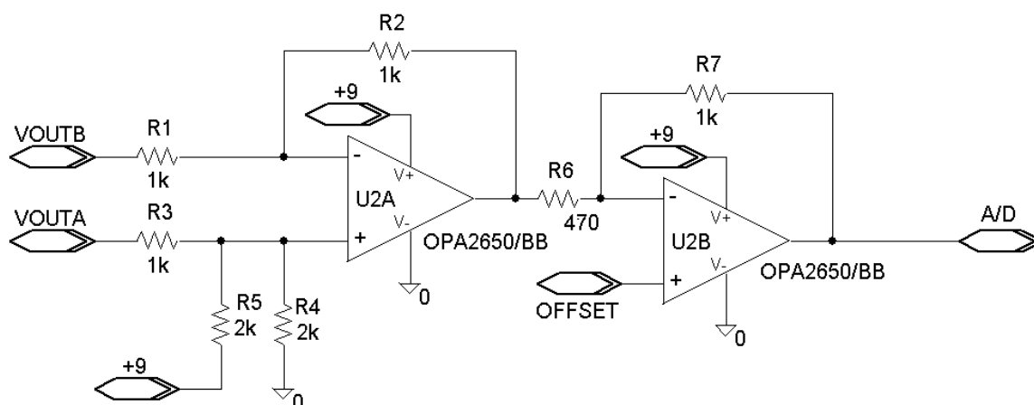
Figure 38. Correlated Double Sampling Output Circuit Block Diagram
