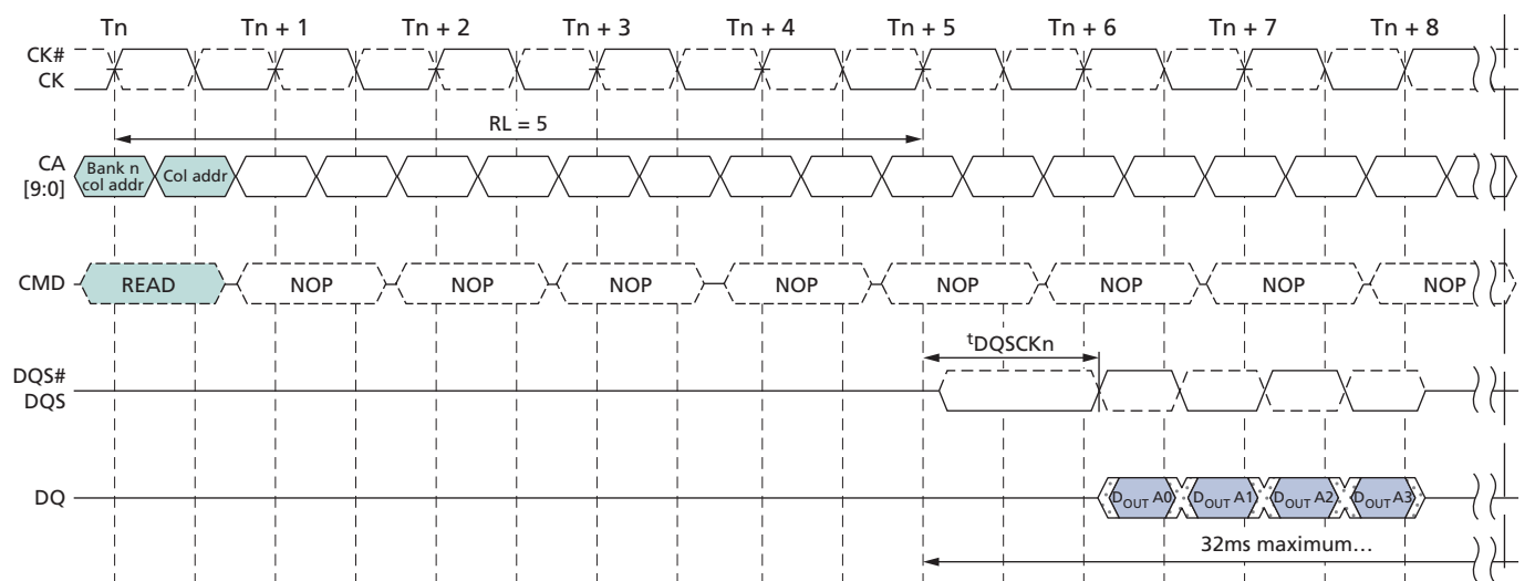
Figure 33: t_{DQSKDL} Timing
