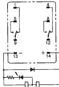
MY2N-D2/MY2IN-D2 (DC Models Only)
