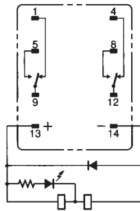
MY2N1-D2/MY2IN1-D2 (DC Models Only)
