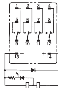
MY4(Z)N-D/MY4(Z)IN-D2 (DC Models Only)
