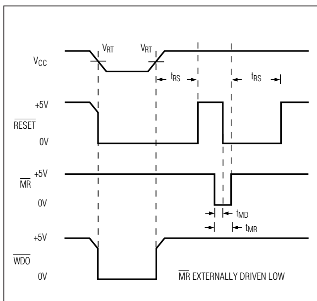
Figure 4. MAX705/MAX706 \overline{\text{RESET}} , \overline{\text{MR}} , and \overline{\text{WDO}} Timing with WDI Three-Styled. The MAX707/MAX708/MAX813L \overline{\text{RESET}} output is the inverse of \overline{\text{RESET}} shown.
