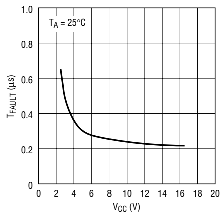
T_{\text{FAULT}} vs V_{CC}
