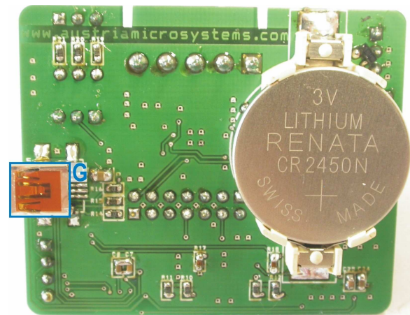
Figure 2: Board Description Bottom – Connectors
