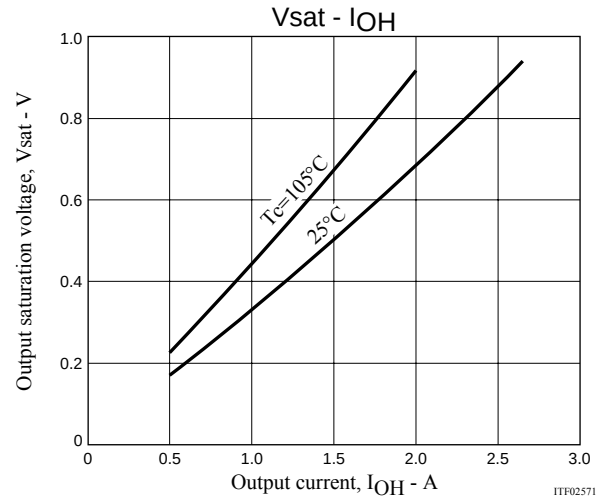
STK672-630C-E Output saturation voltage, V_{sat} - Output current, I_{OH}
