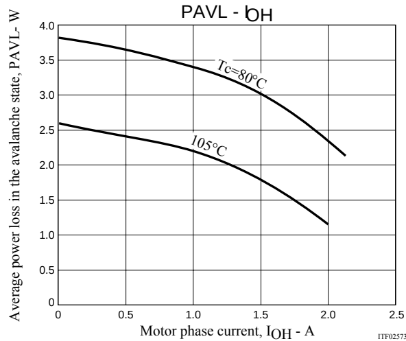
Figure 3 Allowable Loss Range, PAVL - I_{OH} During STK672-630C-E Avalanche Operations
