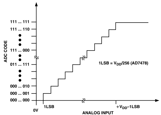
Figure 11. Transfer Characteristic for AD7478
