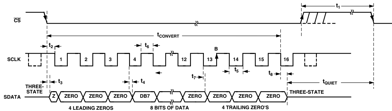
Figure 23. AD7478 Serial Interface Timing Diagram
