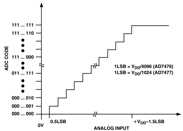
Figure 10. Transfer Characteristic for the AD7476/AD7477
