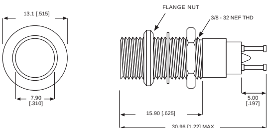
HOLDER WITHOUT COLLAR*
