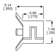
SPEED CLIP 515-0051
