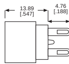
CONNECTOR 515-0074
