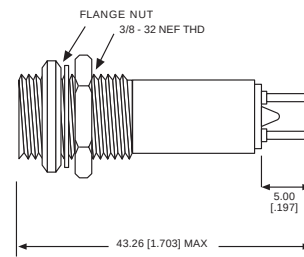
HOLDER WITHOUT COLLAR†
