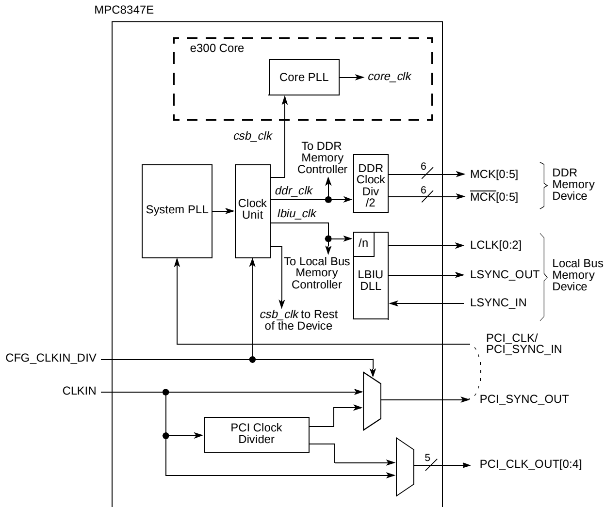
Figure 41. MPC8347E Clock Subsystem
