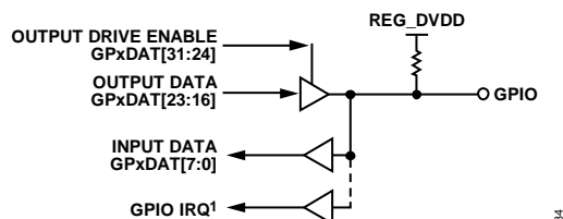
Figure 36. ADuC7032-8L GPIO
