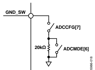
Figure 18. Internal Ground Switch Configuration
