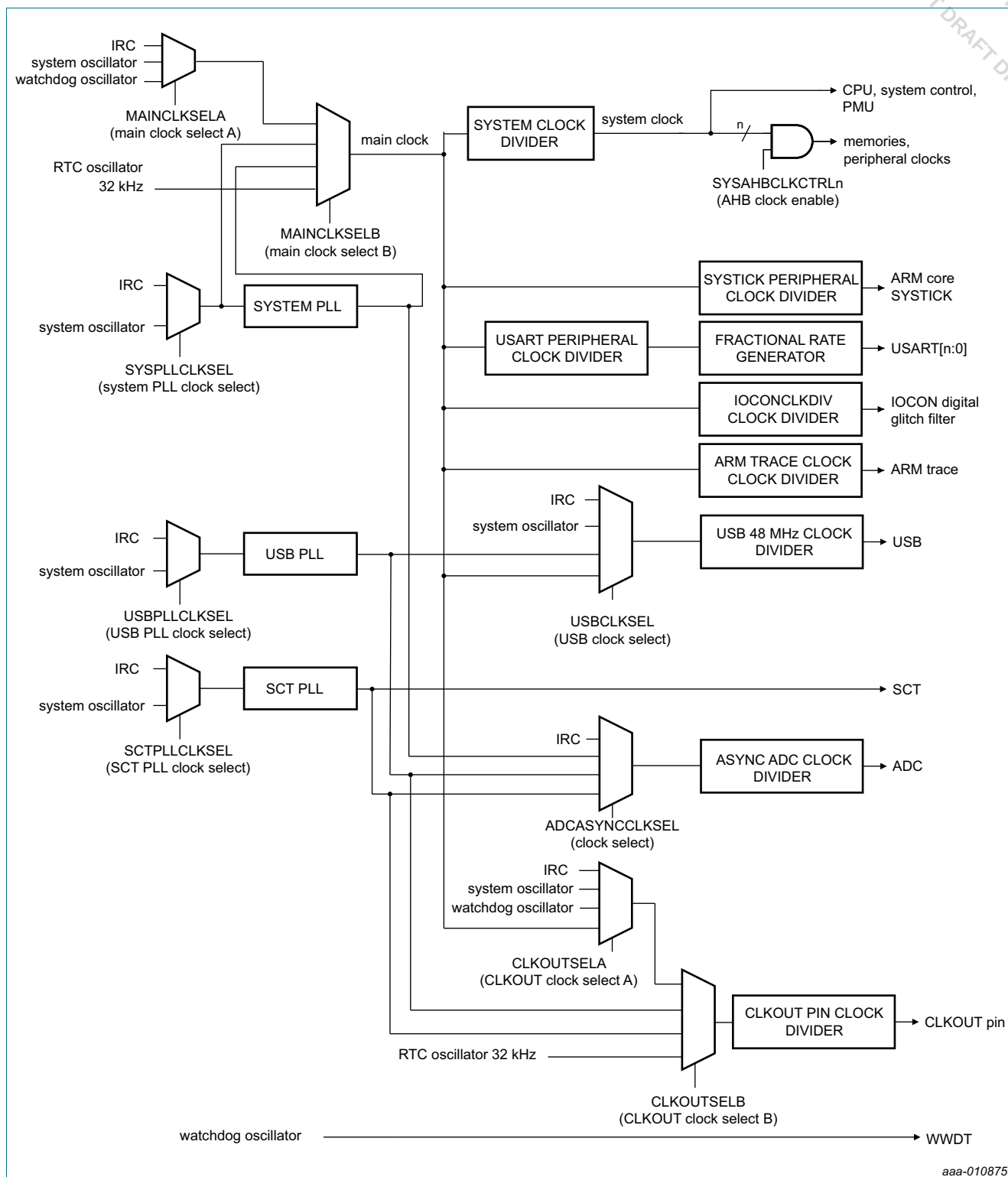
Fig 12. Clock generation
