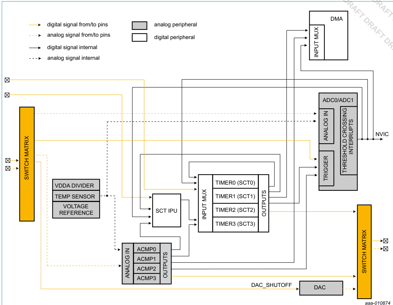
Fig 11. Subsystem with timers, switch matrix, DMA, and analog components
