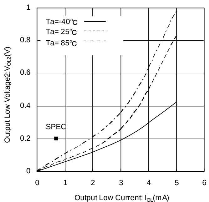
Fig 7. Output Low Voltage 2 vs Output Low Current ( V_{CC} = 1.6\text{V} )
