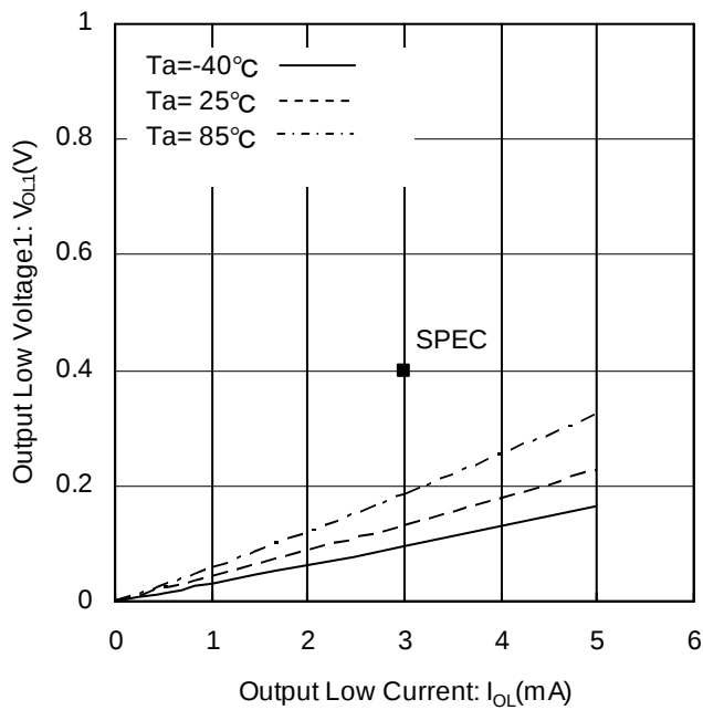
Fig 6. Output Low Voltage 1 vs Output Low Current ( V_{CC} = 2.5\text{V} )
