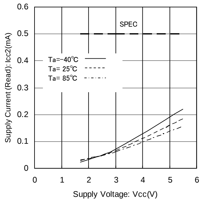
Figure 11. Supply Current (Read) vs Supply Voltage (fsc1=400kHz)
