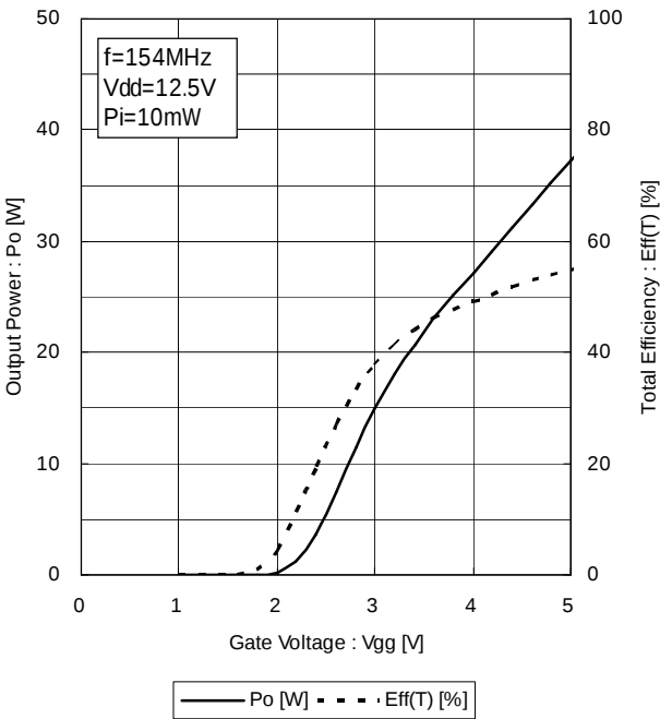
Output Power, Total Efficiency versus Gate Voltage
