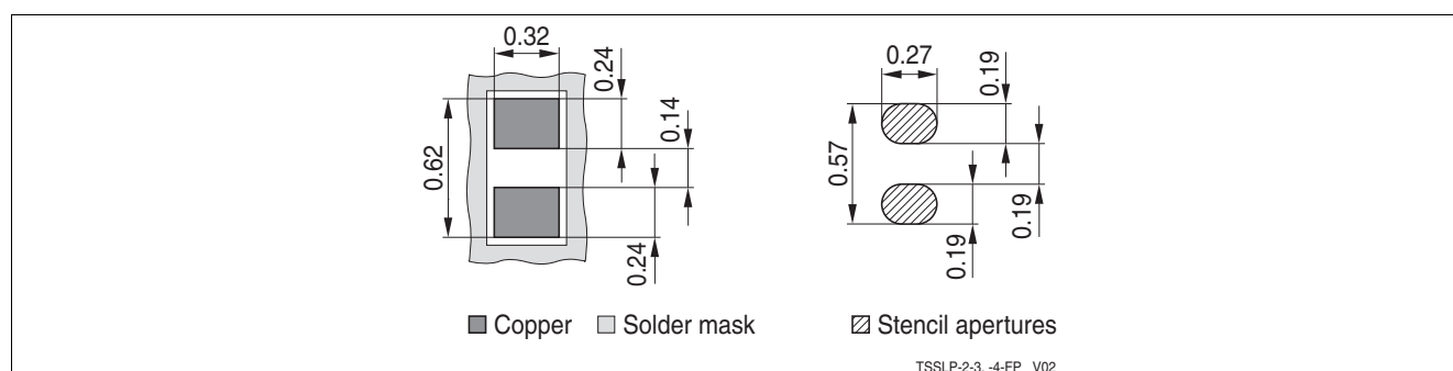
Figure 4-2 TSSLP-2-4: Footprint
