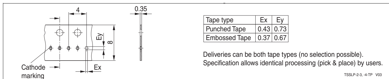
Figure 4-3 TSSLP-2-4: Packing
