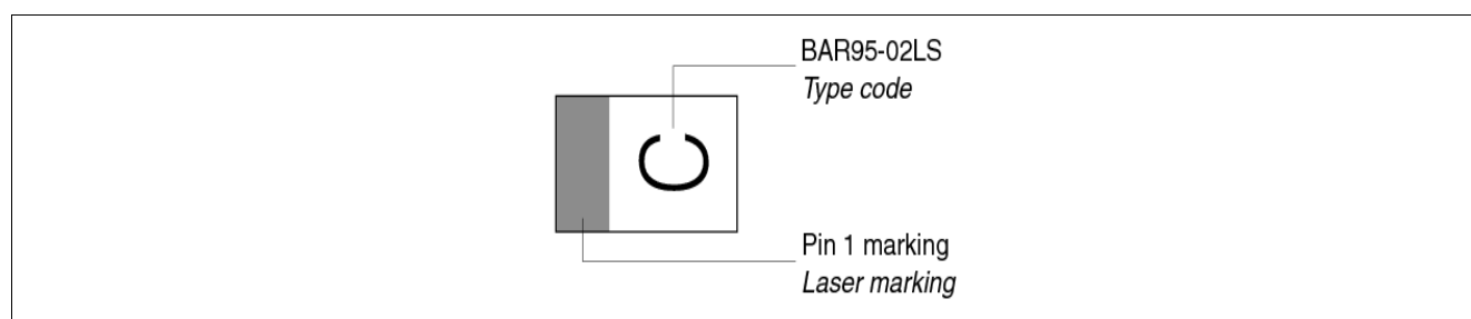
Figure 4-4 TSSLP-2-4: Marking (example)
