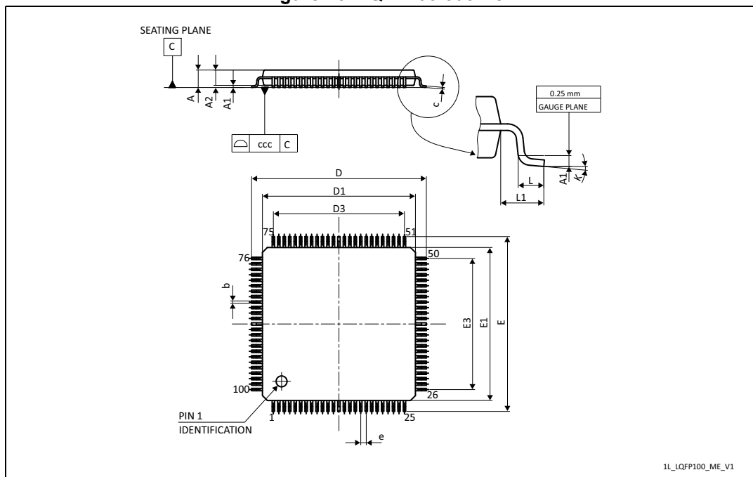
Figure 46. LQFP100 outline
