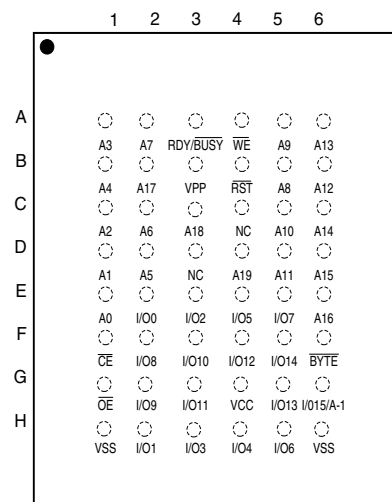
AT49BV162A(T) CBGA Top View (Ball Down)
