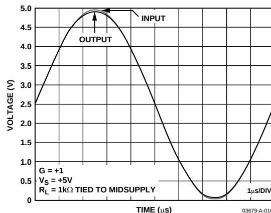
Figure 5. Rail-to-Rail Response
