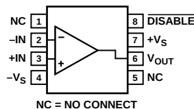
Figure 1. SOIC-8 (R)
