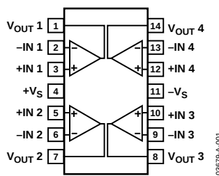
Figure 4. SOIC-14 (R) and TSSOP-14 (RU)
