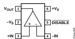
Figure 2. SC70-6 (KS)
