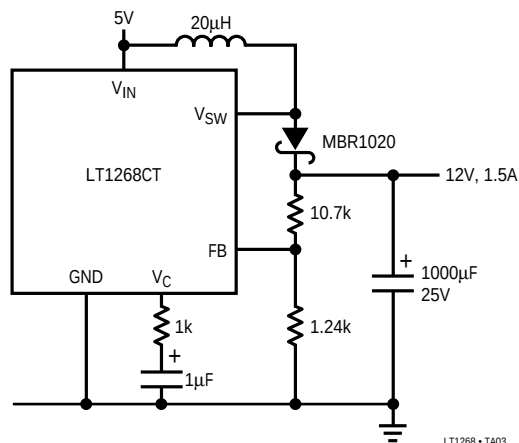
Boost Converter (5V TO 12V)
