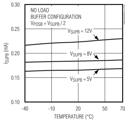
SUPB SUPPLY CURRENT vs. TEMPERATURE
