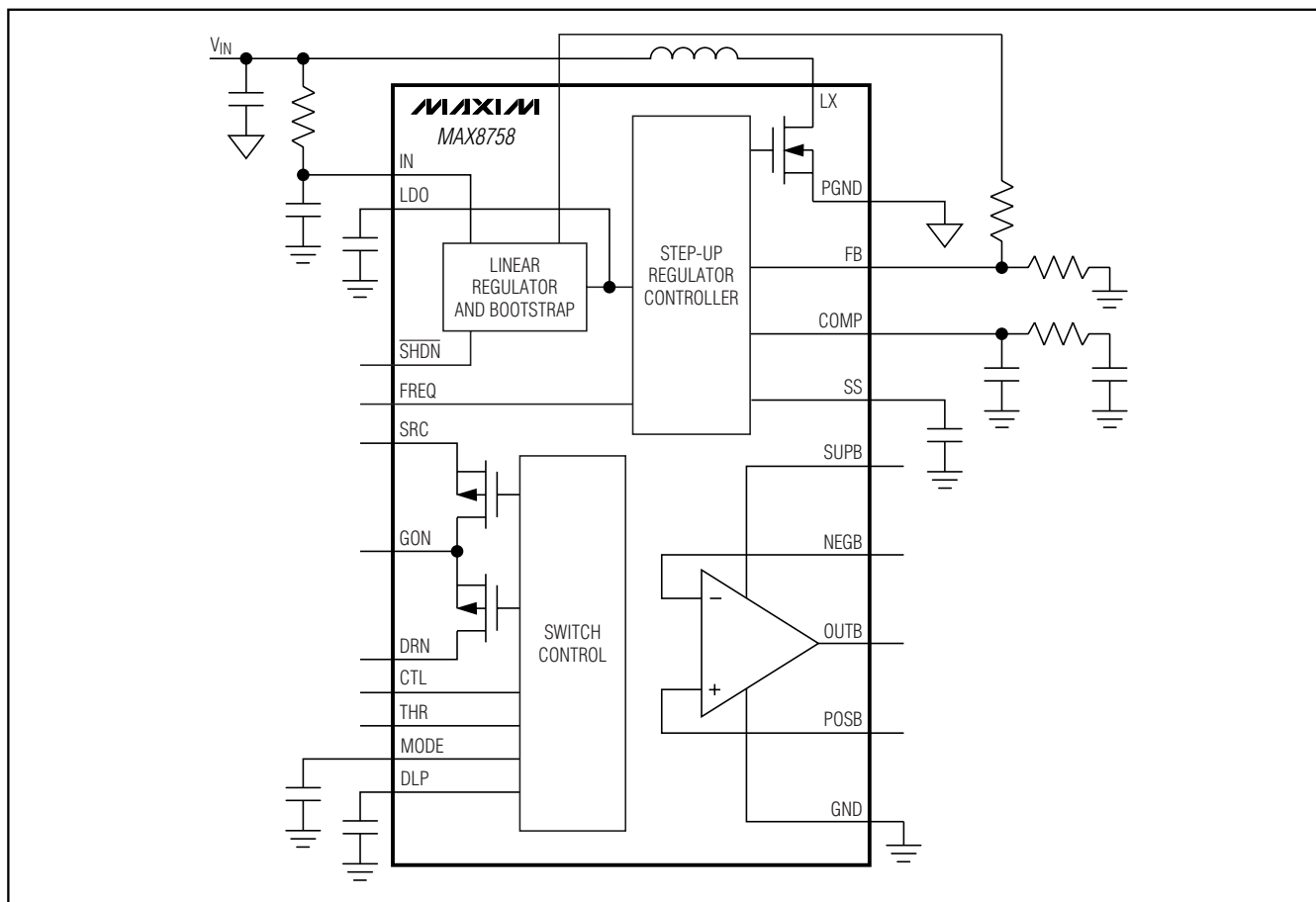
Figure 2. Functional Diagram
