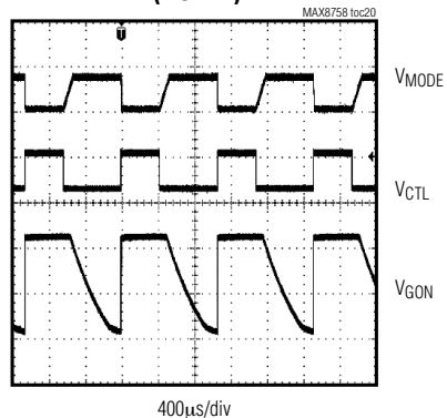
HIGH-VOLTAGE SWITCH CONTROL FUNCTION (MODE 2)
