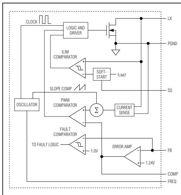
Figure 3. Step-Up Regulator Block Diagram
