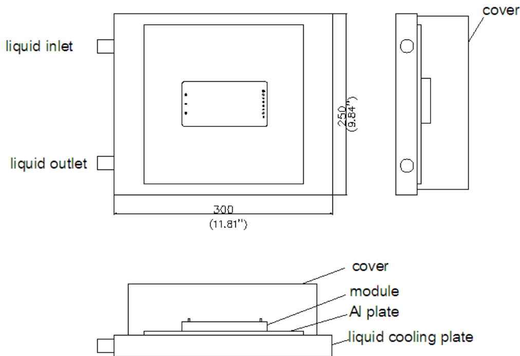
Figure 10: Thermal test setup
