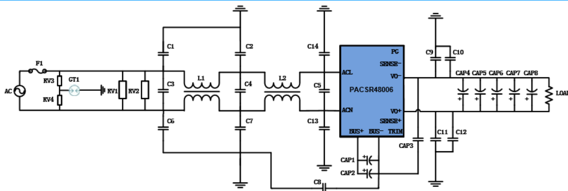
Figure 9: Application connection
