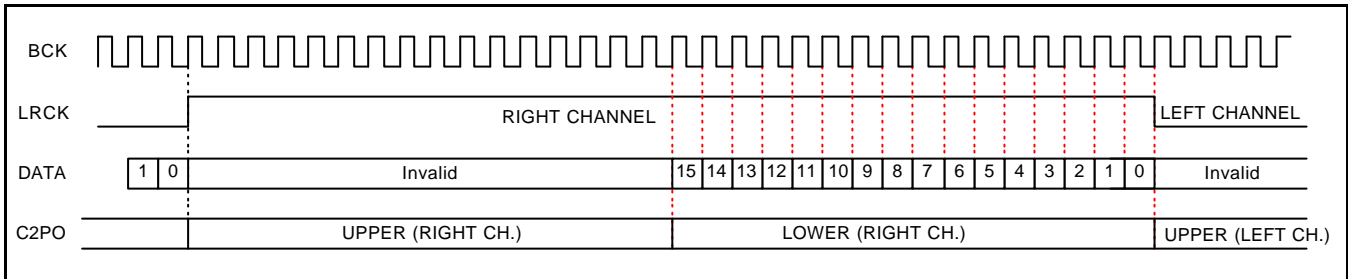
(c) 24-bit BCK, MSB First, Right Channel Low, C2PO MSB First, Data Latch Timing High:
