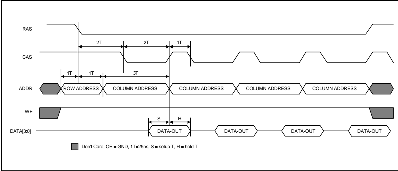
Figure 7. Read Cycle
