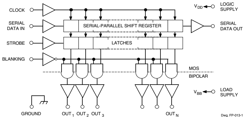
Dwg. FP-013-1
