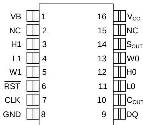
16-Pin SO (300-mil) See Mech. Drawings Section
