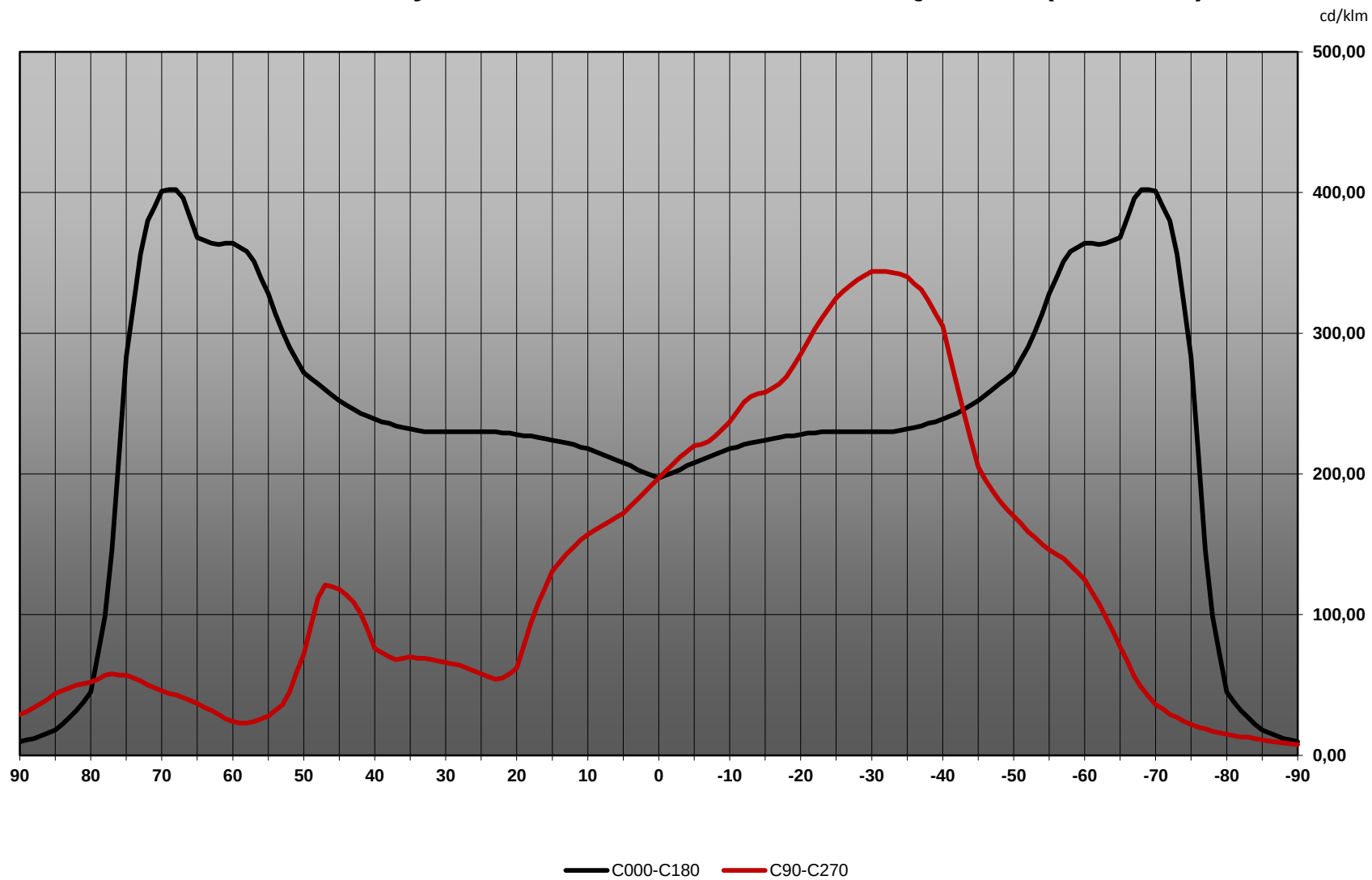
Absolute intensity of C12726&CA12889_STRADA-SQ-T-DWC (Luxeon M)
