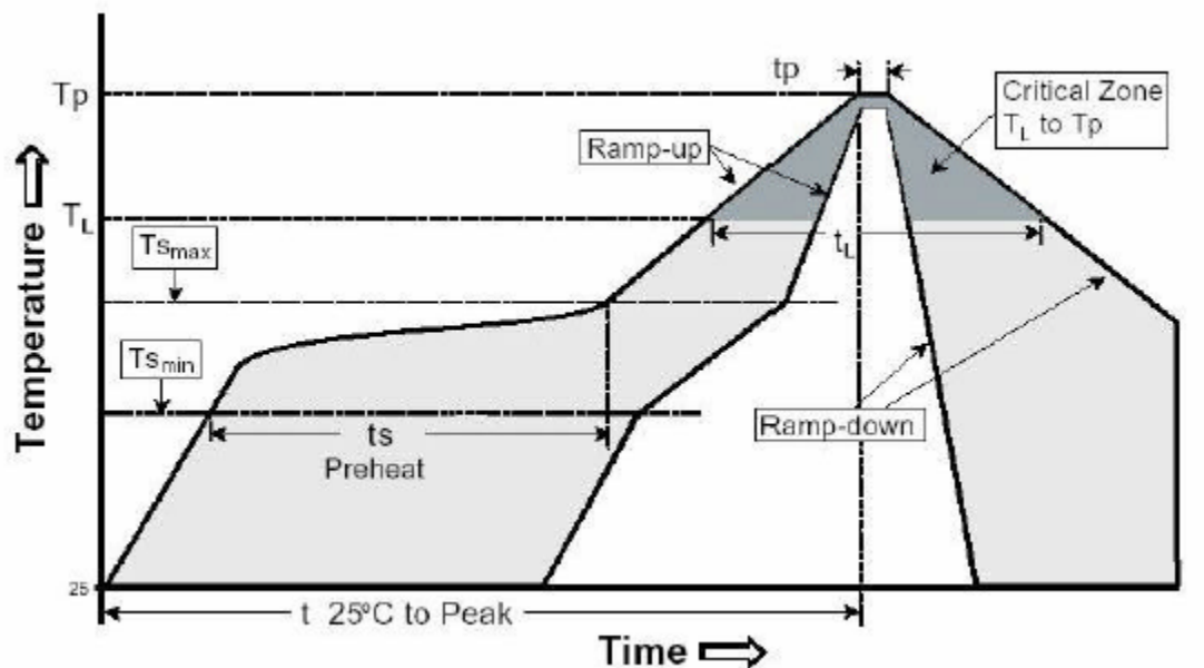
Figure 23. Reflow Profile
