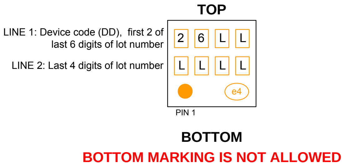
Figure 6.4 PAC1720 Package Marking
