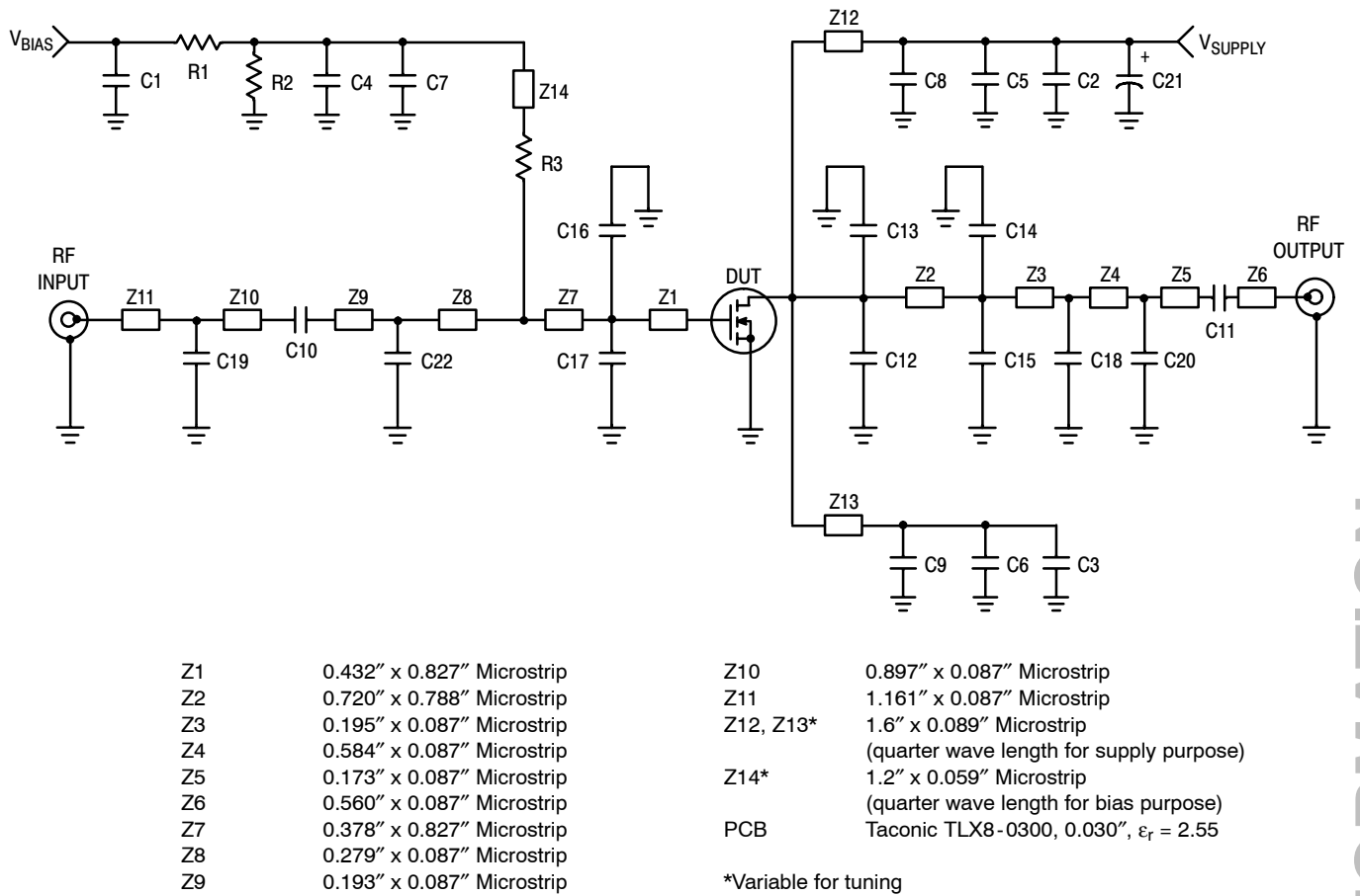
Figure 14. MRF5S9101MR1(MBR1) 800 MHz Test Circuit Schematic
