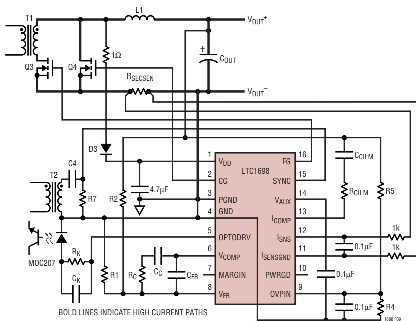
Figure 9. LTC1698 Layout Diagram
