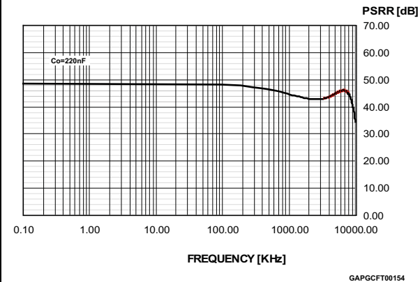
Figure 20. PSRR
