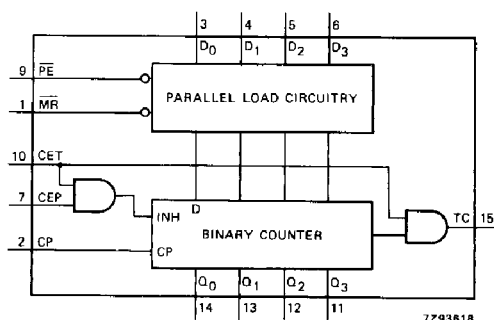
Fig. 4 Functional diagram.
