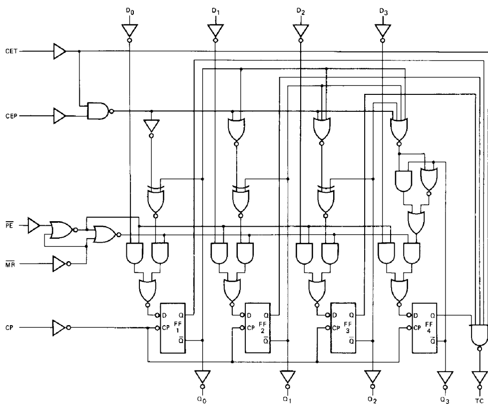
Fig. 7 Logic diagram.
