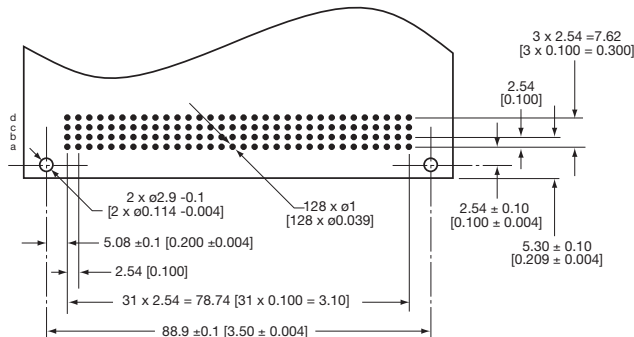
HOLE PATTERN
