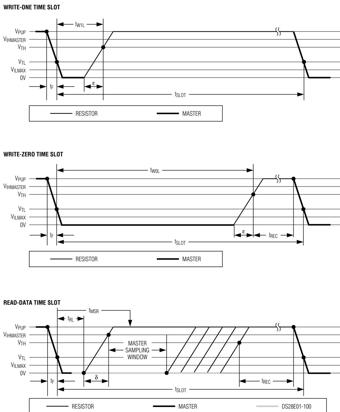
Figure 12. Read/Write Timing Diagrams
