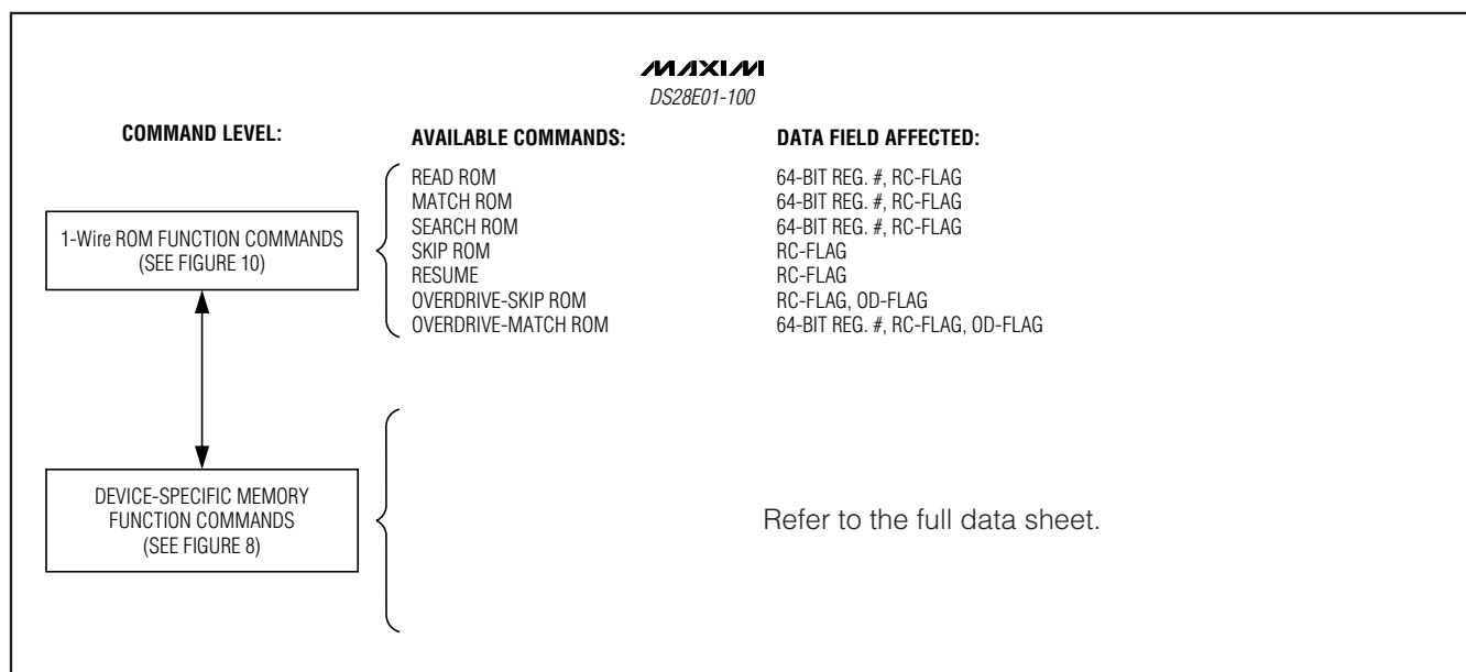
Figure 2. Hierarchic Structure for 1-Wire Protocol
