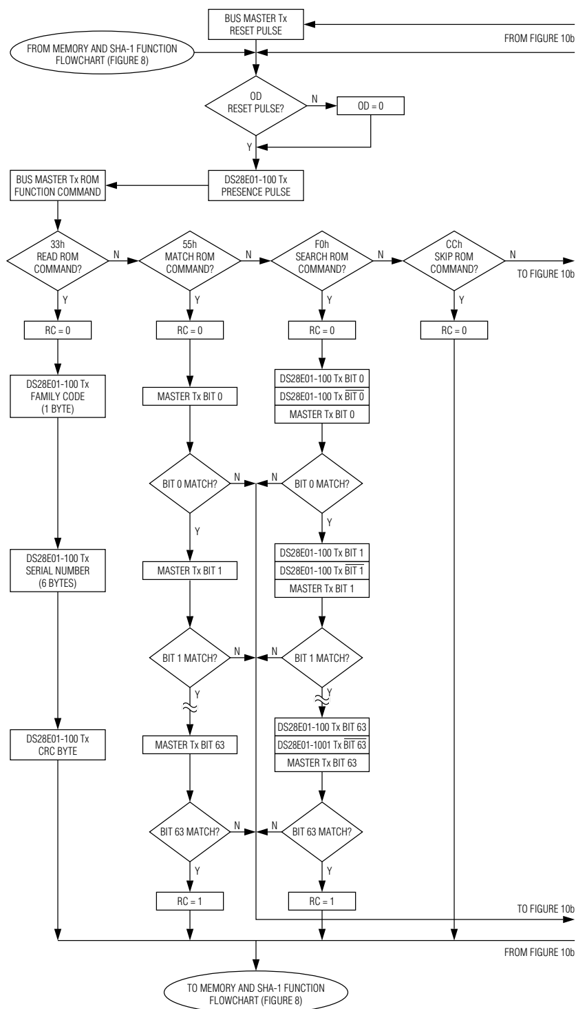
Figure 10a. ROM Functions Flowchart
