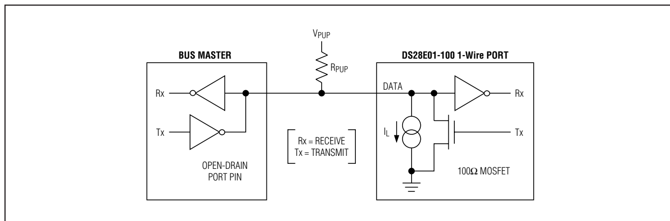
Figure 9. Hardware Configuration
