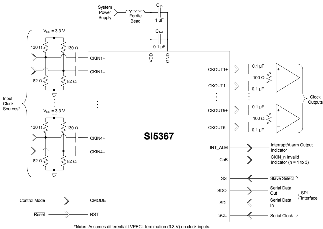
Figure 3. Si5367 Typical Application Circuit (SPI Control Mode)
