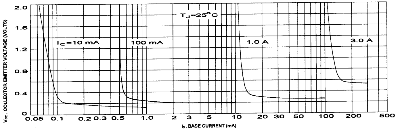
"ON" VOLTAGES
